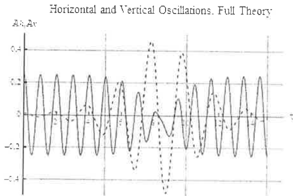
Fig. 3 Mathematica 6.0 plot of the full nonlinear system of equations (I), (II); time evolution of the vertical oscillations (continuous line) and horizontal oscillations (dashed line); k = 50 N/m, \ell = 1 m, m = m_R = 1.274 kg.
