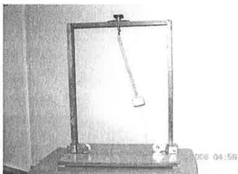
Photograph of the apparatus in action; the instant of maximum horizontal deviation; the flow of water is visible; in this pendulum mode of oscillations, the flow rate depends on the water height in vessel, but otherwise is constant.
