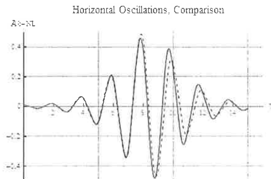
Fig. 5 The comparison of solutions for horizontal oscillations; exact theory (continuous line) and linear theory (dashed line); k = 50 \text{ N/m} , \ell = 1 \text{ m} , m = m_r = 1.274 \text{ kg} .
