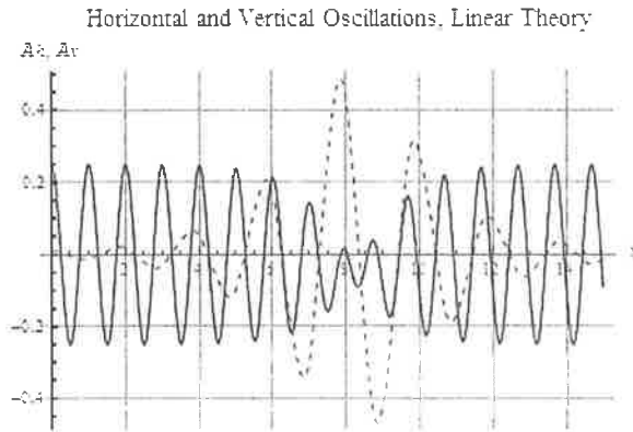
Fig. 4 Mathematica 6.0 plot of the linearized system of equations (I- \ell ), (II- \ell ); time evolution of the vertical oscillations (continuous line) and horizontal oscillations (dashed line); k = 50 \text{ N/m} , \ell = 1 \text{ m} , m = m_r = 1.274 \text{ kg} .
